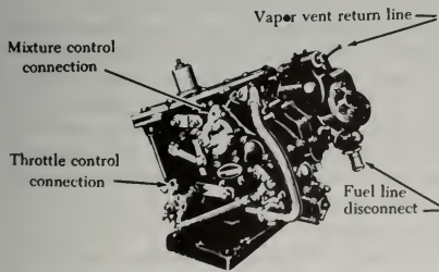
FIGURE 3-40. Carburetor installation connecting points.
